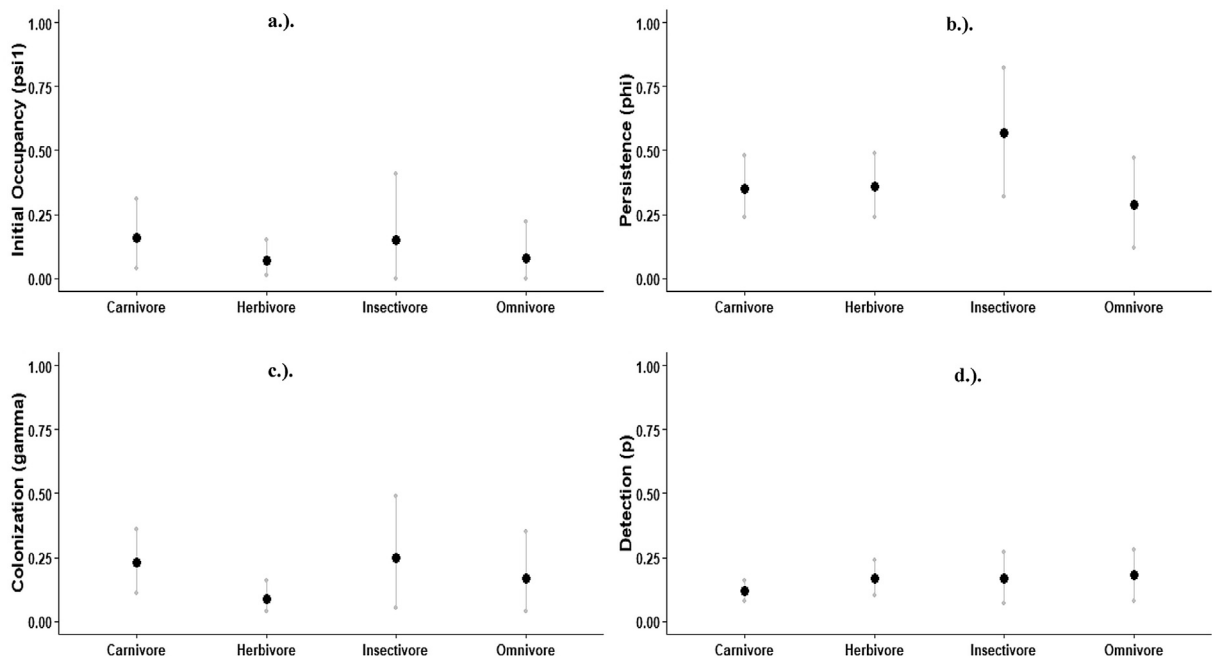
Fig. 3. Bar-plots of estimated mean detectability, occupancy, persistence and colonization of four dietary guilds in Nam Et - Phou Louey National Protected Area, Laos, during 2013–2017.
