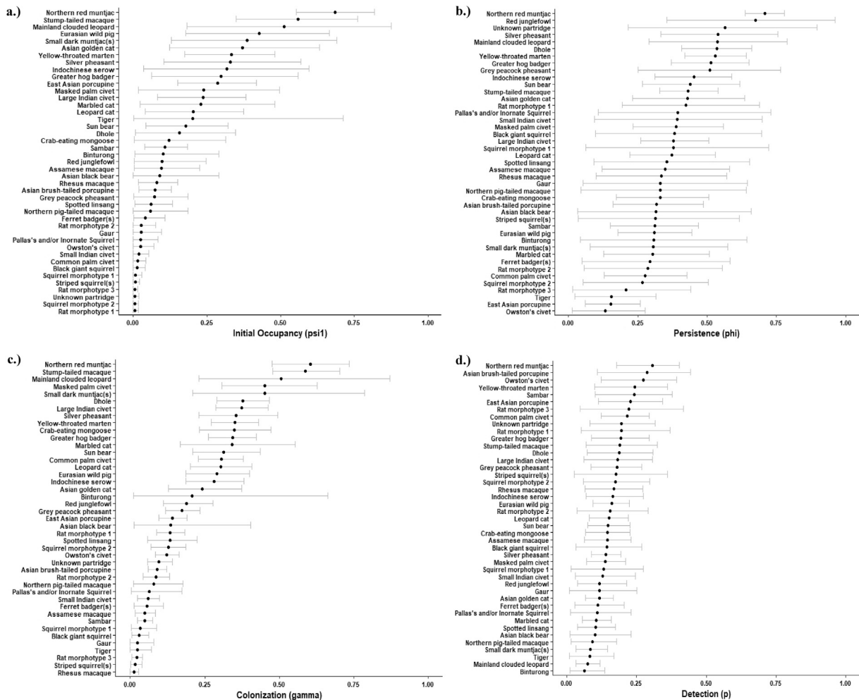
Fig. 2. Bar-plots of estimated mean detectability, occupancy, persistence and colonization of species detected in Nam Et - Phou Louey National Protected Area, Laos, during 2013–2017.
